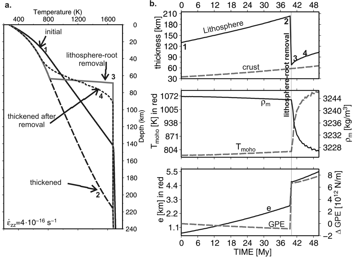
Figure 2. (a) Time evolution of a geotherm under constant thickening ( \dot{\epsilon}_{zz} = 4. \times 10^{-16} \text{ s}^{-1} ) and at different stages: curve 1, initial; curve 2, after 40 m.y. of constant thickening; curve 3, after removal of the lithospheric mantle; and curve 4, 2 m.y. after the lithospheric removal, resulting from conduction and constant thickening. (b) Time evolution of: lithosphere and crustal thickness; Moho temperature and lithospheric mantle density; elevation and changes in gravitational potential energy ( \Delta \text{GPE} = \text{GPE}(t) - \text{GPE}(t = 0) ).
