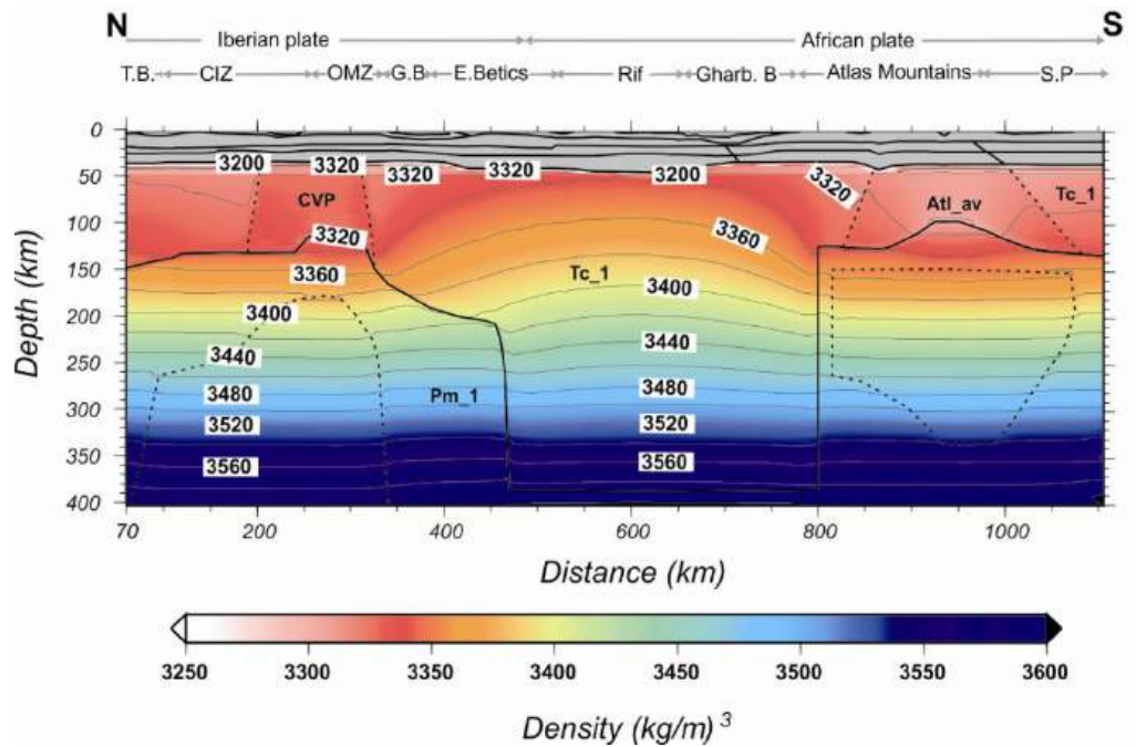
Figure 5.7: Calculated mantle density distribution along the Iberian Massif–Arc of Gibraltar–Atlas Mountains geo-transect. Contour lines every 20 kg m -3 .
