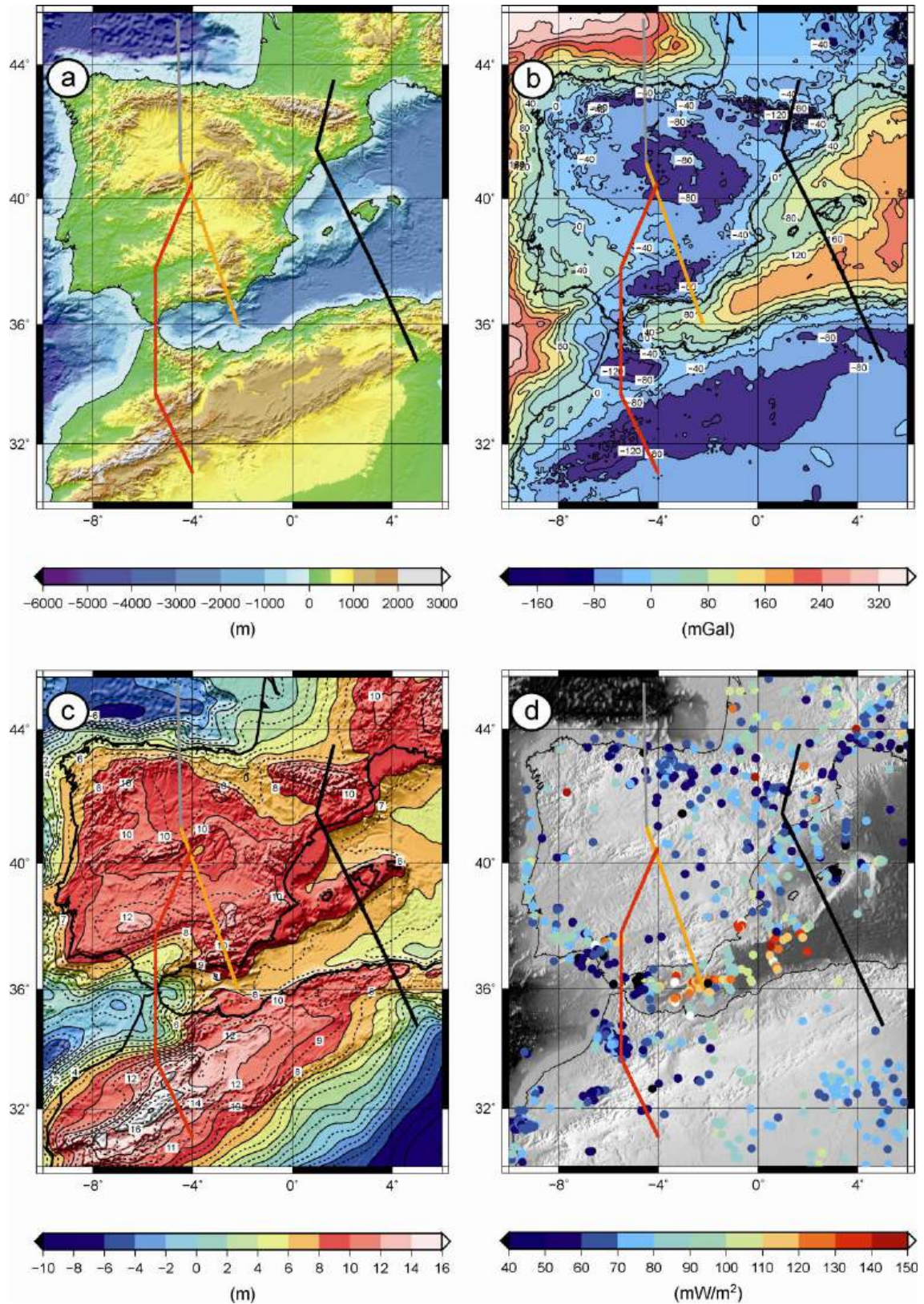
Figure 1.5: Geophysical data. a) Elevation map from ETOPO Global Data Base (V9.1) ( http://www.ngdc.noaa.gov/mgg/fliers/01mgg04.html ). b) Bouguer anomaly. Onshore, in the Iberian Peninsula, the Bouguer anomaly comes from Ayala (2013). Offshore and Africa Bouguer anomaly has been calculated from the free air anomaly by Sandwell and Smith (1997) using Fullea et al. (2008).
