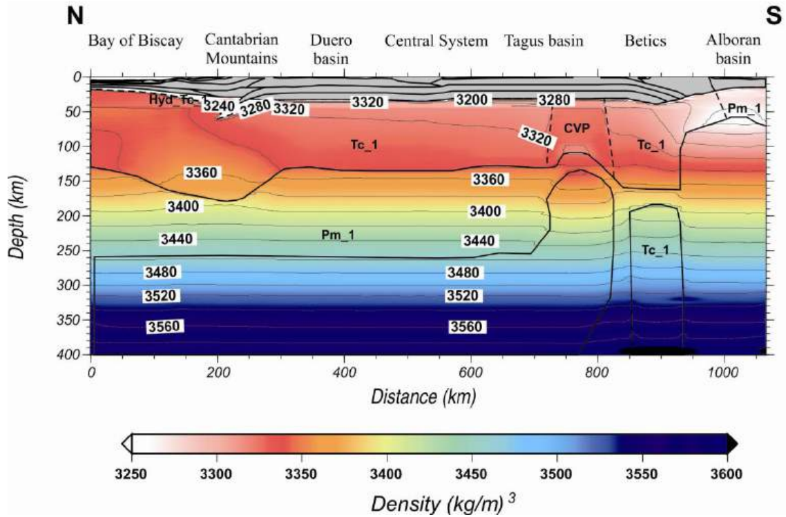
Figure 4.6: Calculated mantle density distribution along the geo- transect. Contour lines every 20 \text{ kg m}^{-3} .
