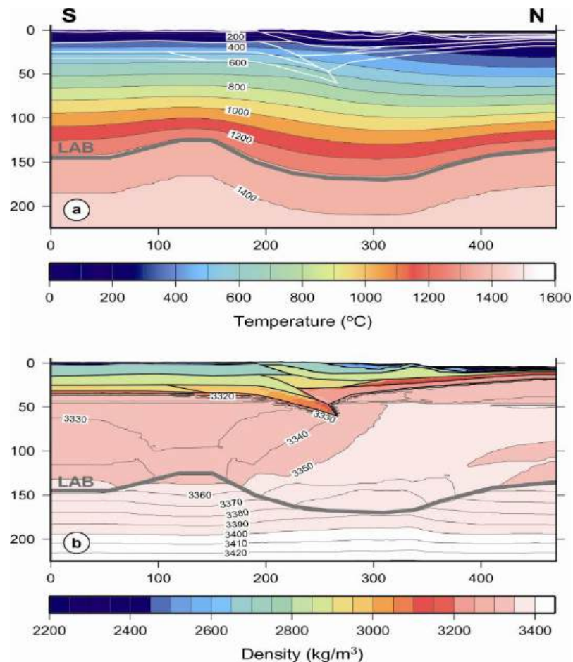
Figure 3.5: a) Thermal and b) density structure along the modeled transect. The grey bold line (LAB) represents the base of the thermal lithosphere.
