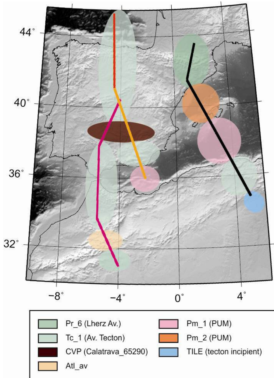
Figure 6.2: Topographic map of the study area showing the lithospheric mantles compositions used in this thesis. Thick lines locate the modeled transects: Black line-first geo-transect; Red line-second geo-transect; Light orange line-third geo-transect and pink line-fourth geo-transect. Chemical compositions described in Table 2.2, Table 3.2, Table 4.2 and Table 5.2.
