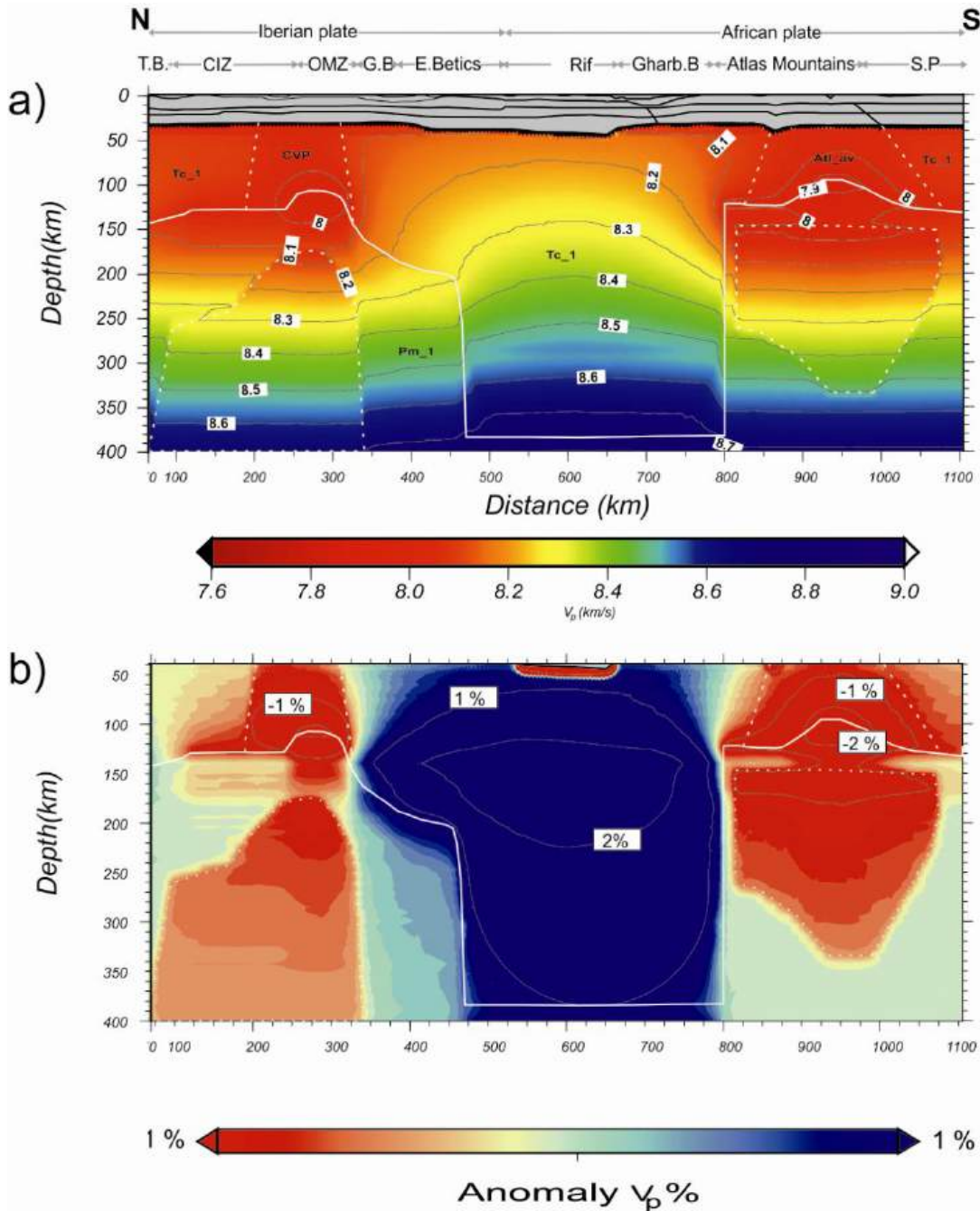
Figure 5.8. a) Calculated P-wave seismic velocities in the upper mantle down to 400 km; b) synthetic P-wave tomography from our model. In this case velocity anomalies are relative to the synthetic reference model (reference model consisting of a 130-km thick lithosphere and 30-km thick crust with a lithosphere mantle composition corresponding to Tc_1.) (see text). Contour lines every 1%. Compare with Figure 5.2.
