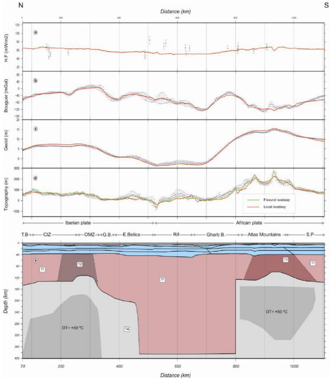
Figure 5.4: Model results (red lines), measured data with the standard deviation of data projected onto the profile within a strip of 25 km half-width (blue dots and vertical bars): (a) surface heat flow; (b) Bouguer anomaly; (c) geoid height; (d) elevation and coupled calculated topography under local isostasy (red line) and under regional isostasy with elastic thickness varying between 20 and 10 km (green line); (e) lithospheric structure. Crustal structure like in Fig. 5.2. Numbers in panel (e) denote mantle bodies summarized in Table 5.2. Dataset sources as in Fig. 1.3.
