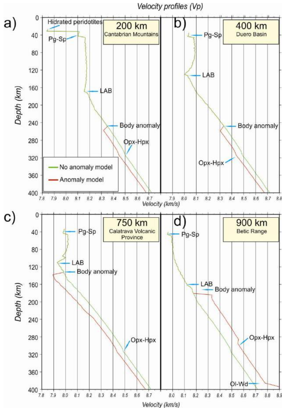
Figure 4.11: Depth variation of P-wave velocities calculated in the preferred model along the profile (at 200, 400, 750 and 900 km distance) for model with the sub-lithospheric anomalous body (red line) and model without the anomalous body (green line). Arrows denote the lithosphere-asthenosphere boundary (LAB) and the following phase transitions: Pg-Sp, plagioclase-spinel; Opx-Hpx, orthopyroxene-high-pressure magnesian pyroxene.
