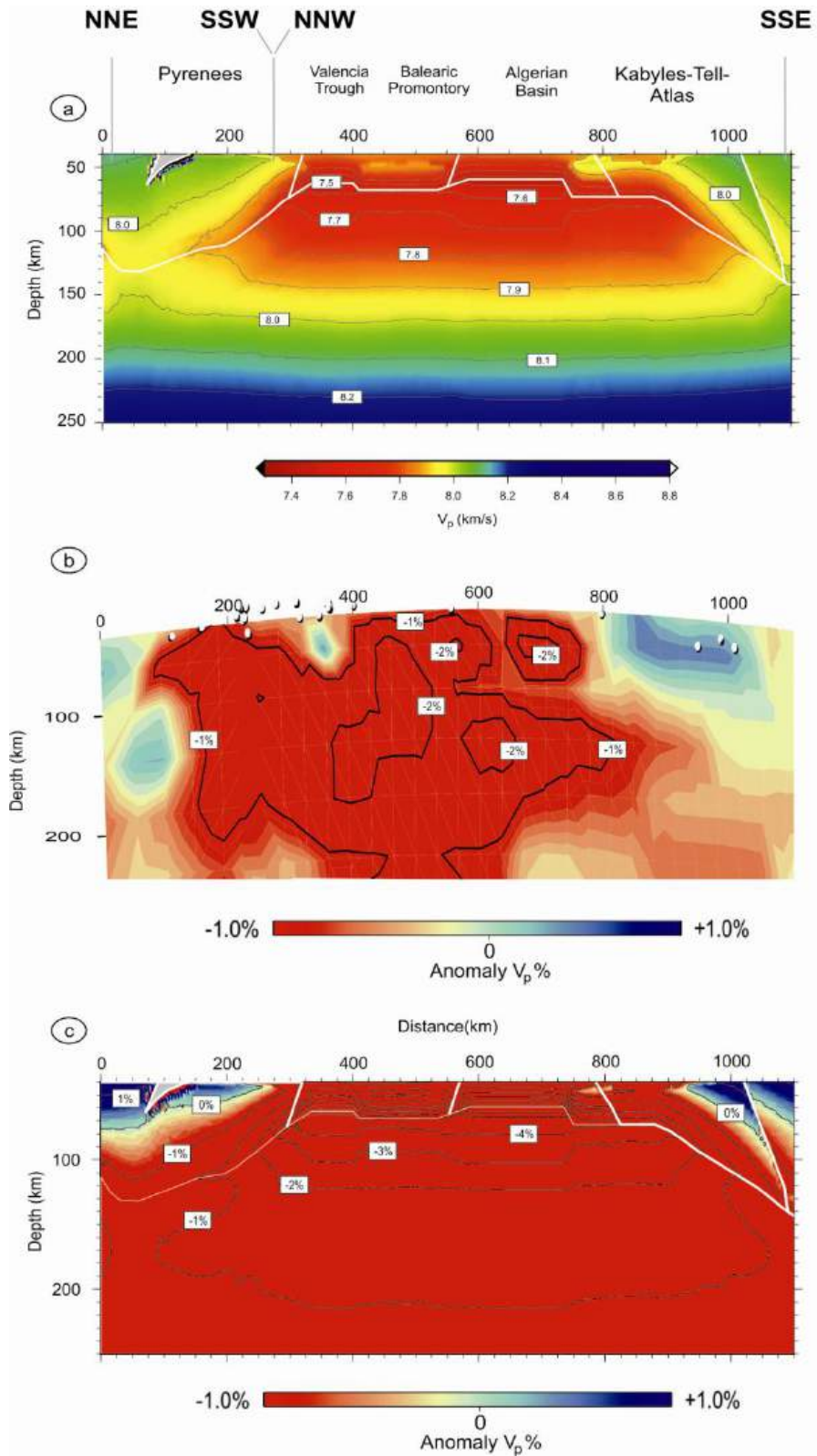
Figure 2.8: a) Calculated P-wave seismic velocities in the upper mantle (calculations extend down to 400 km depth). White solid lines indicate mantle domains with different chemical composition. b) P-wave tomography model (Villaseñor et al., 2003) and c) synthetic P-wave tomography from our model. In both cases velocity anomalies are relative to the ak135 reference model (Kennett et al., 1995). Contour lines every 1%.
