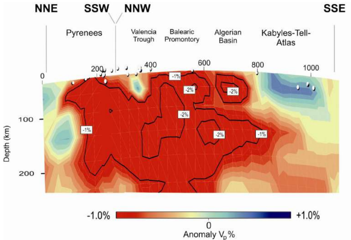
Figure 2.3: P-wave tomography model along the profile (Villaseñor et al., 2003).
