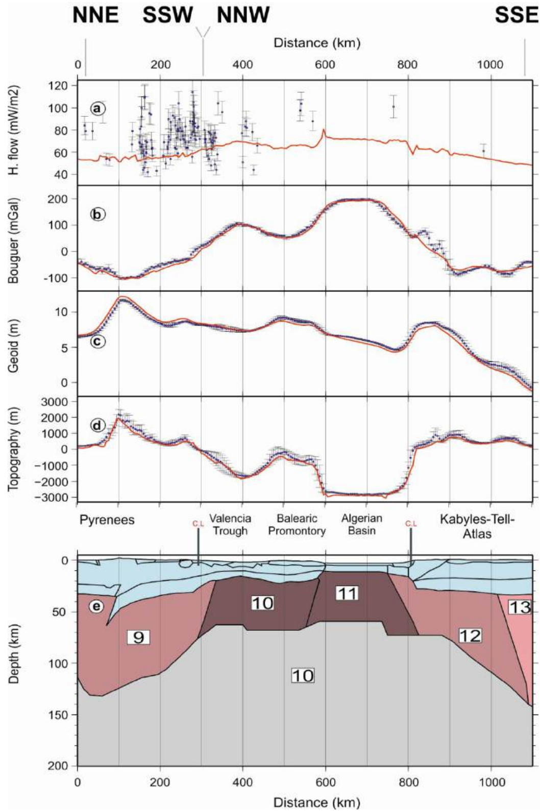
Figure 2.4: Model results (red lines) and measured data with the standard deviation of data projected onto the profile within a strip of 25 km half-width except heat flow that is projected onto a 50 km half-width strip (blue dots and vertical bars): (a) surface heat flow; (b) Bouguer anomaly; (c) geoid height; (d) elevation; (e) lithospheric structure. Crustal structure as in Fig. 2.2. Numbers in panel (e) denote mantle bodies summarized in Table 2.2. Dataset sources as in Fig. 1.3.
