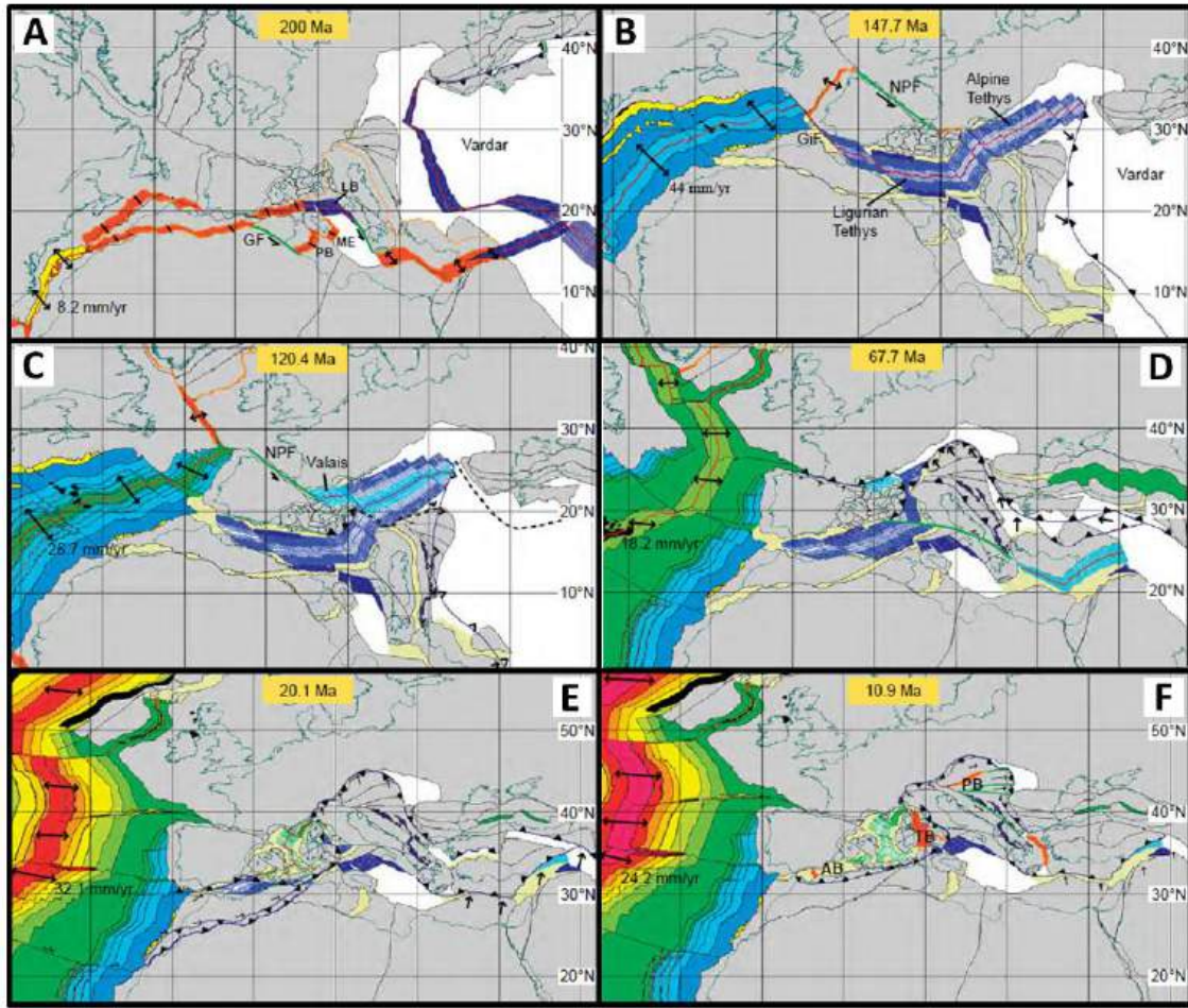
Figure 7.1: Plate tectonic maps showing the evolution of Africa, Iberia and Europe from early Jurassic to late Miocene according to Schettino and Turco (2010). Adapted from Schettino and Turco (2010).
