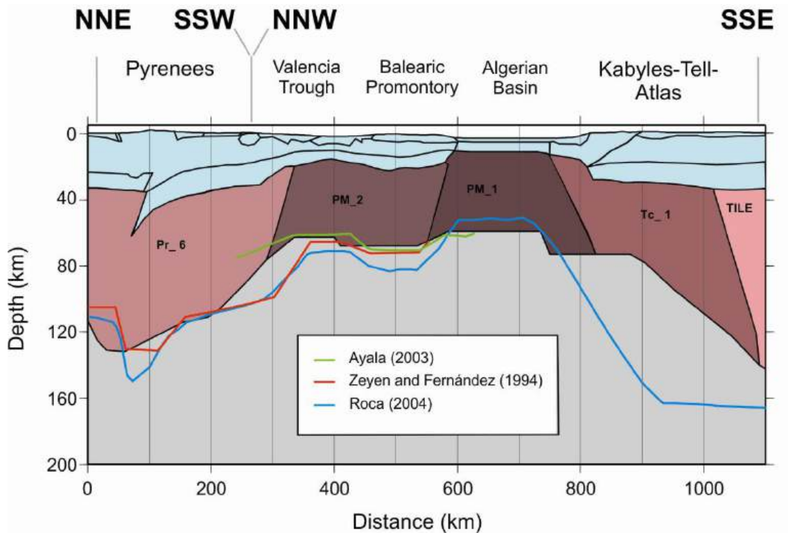
Figure 2.5: Lithosphere structure of the best fit model and mantle domains with different chemical composition (see Table 2.2). Color lines denote LAB geometries proposed in previous studies.
