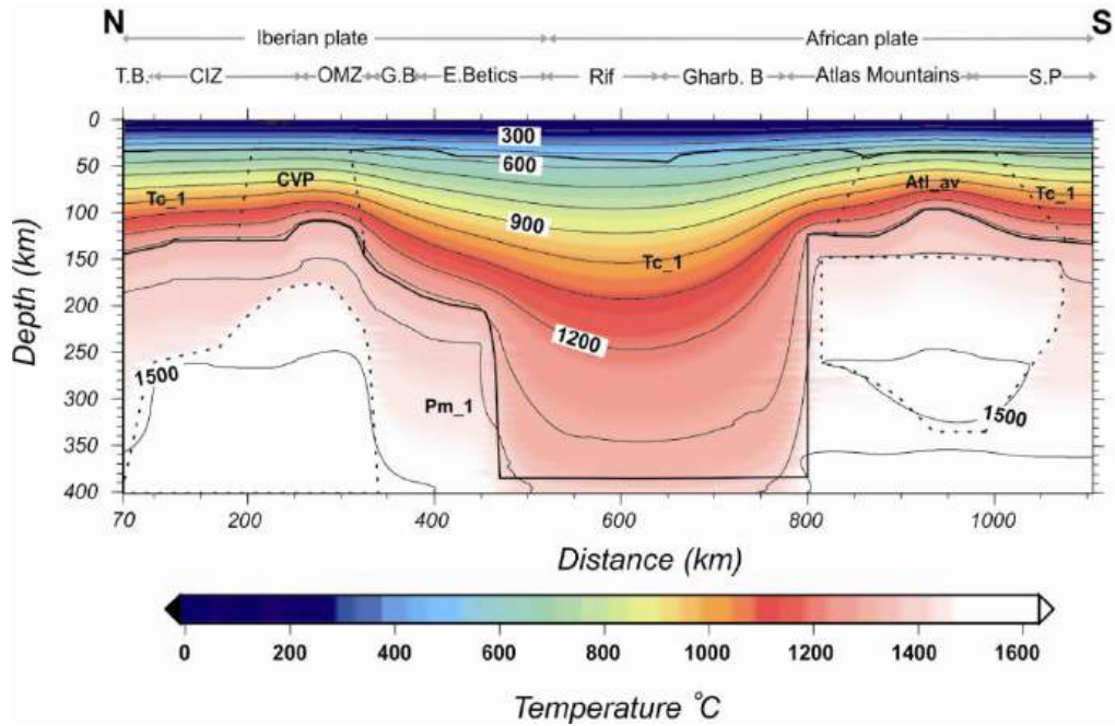
Figure 5.6: Calculated temperature distribution along the Iberian Massif-Arc of Gibraltar-Atlas Mountains geo-transect and mantle domains with different chemical composition (see Table 5.2). Contour lines every 100 °C.
