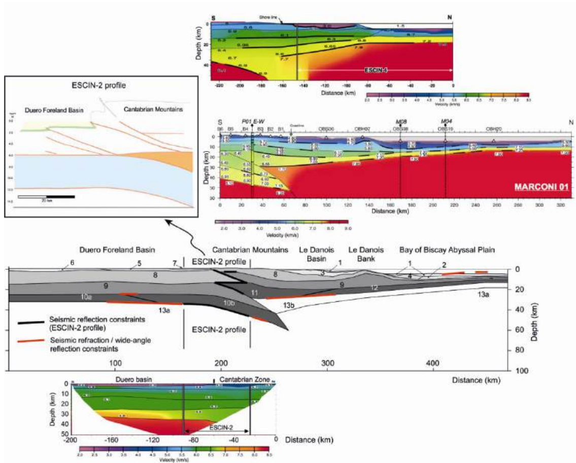
Figure 3.2: Seismic constraints used to delineate the crustal structure of the lithospheric model. Top right panels: P-wave velocity models for the ESCIN-4 and MARCONI-1 profiles (location in Figure 3.1), from Fernández-Viejo et al. (1998) and Ruiz et al. (in prep.), respectively. Superimposed on the MARCONI-1 profile there is a velocity-depth column corresponding to the intersecting E-W Profile 1 of Pedreira et al. (2003, 2007). Note the thin crust beneath the abyssal plain, with velocities of \sim 7.2 km/s in the lower crust (HVLC), and the velocities of 7.8-7.9 km/s in the uppermost mantle, decreasing to \sim 7.7 km/s in the mantle wedge above the north-Iberian crustal root (see text for details). Top left panel: record sections of seismic stations 21 (close to the coast) and 25 (near the Duero Basin), during the acquisition of the ESCIN-4 profile, taken from Gallart et al. (1997). Observe that station 21 records a clear PmP reflection denoting a sharp interface at the base of the HVLC beneath Le Danois Bank and the continental platform, gently dipping towards the south. Station 25, on the other hand, records the presence of this same interface (Bay of Biscay Moho) as south as the coastline, as well as a later PmP' phase interpreted to be produced in the north-dipping Iberian Moho. Middle panel: sketch of the crustal structure of the model with the seismic constraints superimposed: red lines mark clear seismic refraction/wide-angle reflection interfaces; black lines depict the geometrical attitude of reflectors in the ESCIN-2 profile, according to Pulgar et al. (1995) and Gallastegui (2000). Lower panel: P-wave velocity model for Profile 5 (location in Figure 3.1) from Fernández-Viejo et al. (2000), showing the typical Variscan crustal structure of the crust beneath the Duero Basin, with upper, middle and lower crustal levels and a total thickness of 32-35 km. Note the increasing seismic velocities in the lower crust to the south (see text for details).
