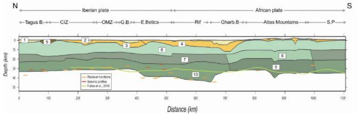
Figure 5.2: Crustal structure corresponding to the best fitting model. Different bodies have been modeled using geological cross-sections and seismic experiments (see text for details). Physical properties of crustal bodies are reported in Table 5.2. CIZ, Central Iberian Zone; OMZ, Ossa Morena Zone; GB, Guadalquivir Basin; S.P, Sharan Platform.
