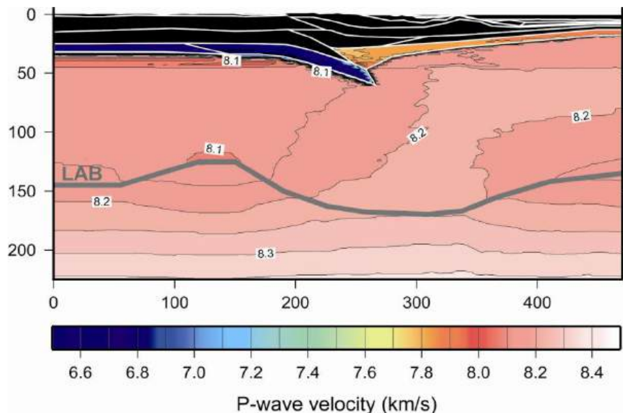
Figure 3.6: P-wave velocity structure along the modeled transect. The grey bold line (LAB) represents the base of the thermal lithosphere.
