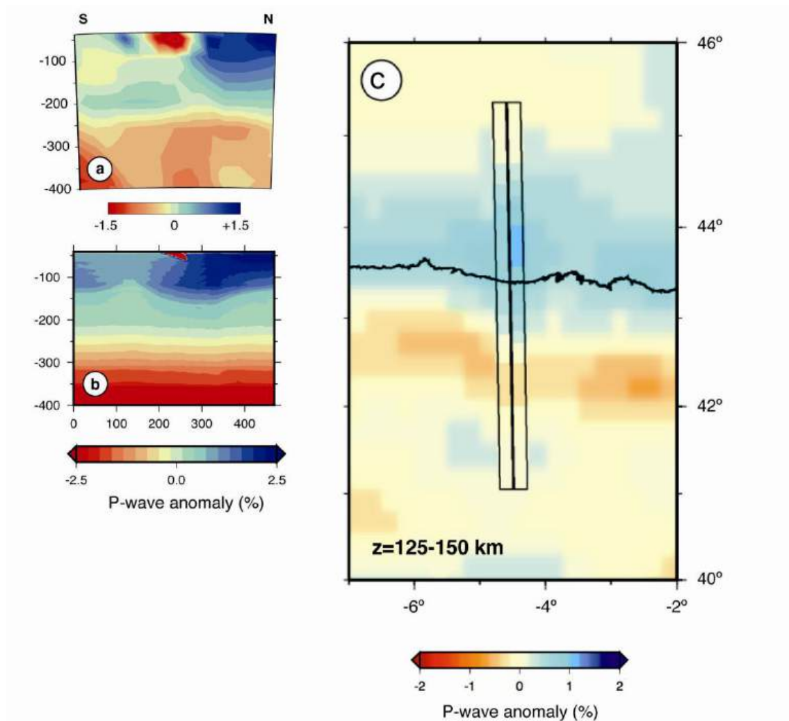
Figure 3.8: Comparison between the P-wave velocity structure calculated for the mantle along the transect
