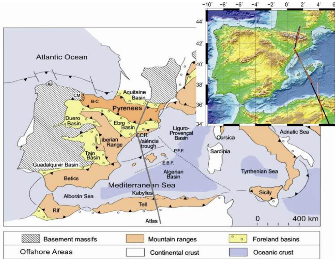
Figure 2.1: Geological map of the study area showing the principal geological domains of Iberia, Western Mediterranean and North Africa (modified from Vergés and Sàbat et al., 1999). Thick gray line locates the modeled transect. Upper right inset shows the main topography and bathymetry features of the study area in which is located: Black line—model transect; Deep blue—ECORS Pyrenees; Yellow— ESCI Catalanides; Green line—ESCI València; Pink line: ALE-4 and dark gray—other seismic experiments (Díaz et al., 2013).
