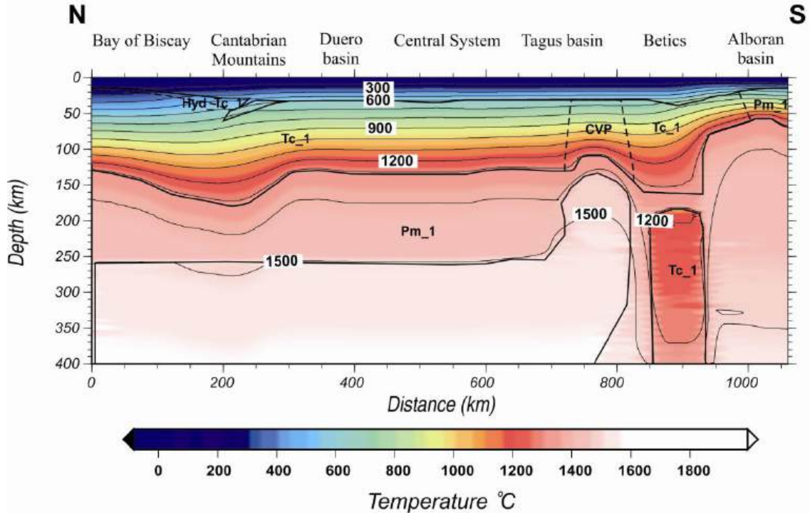
Figure 4.5: Calculated temperature distribution along the geo-transect and mantle domains with different chemical composition (see Table 4.2). Contour lines every 100 °C.
