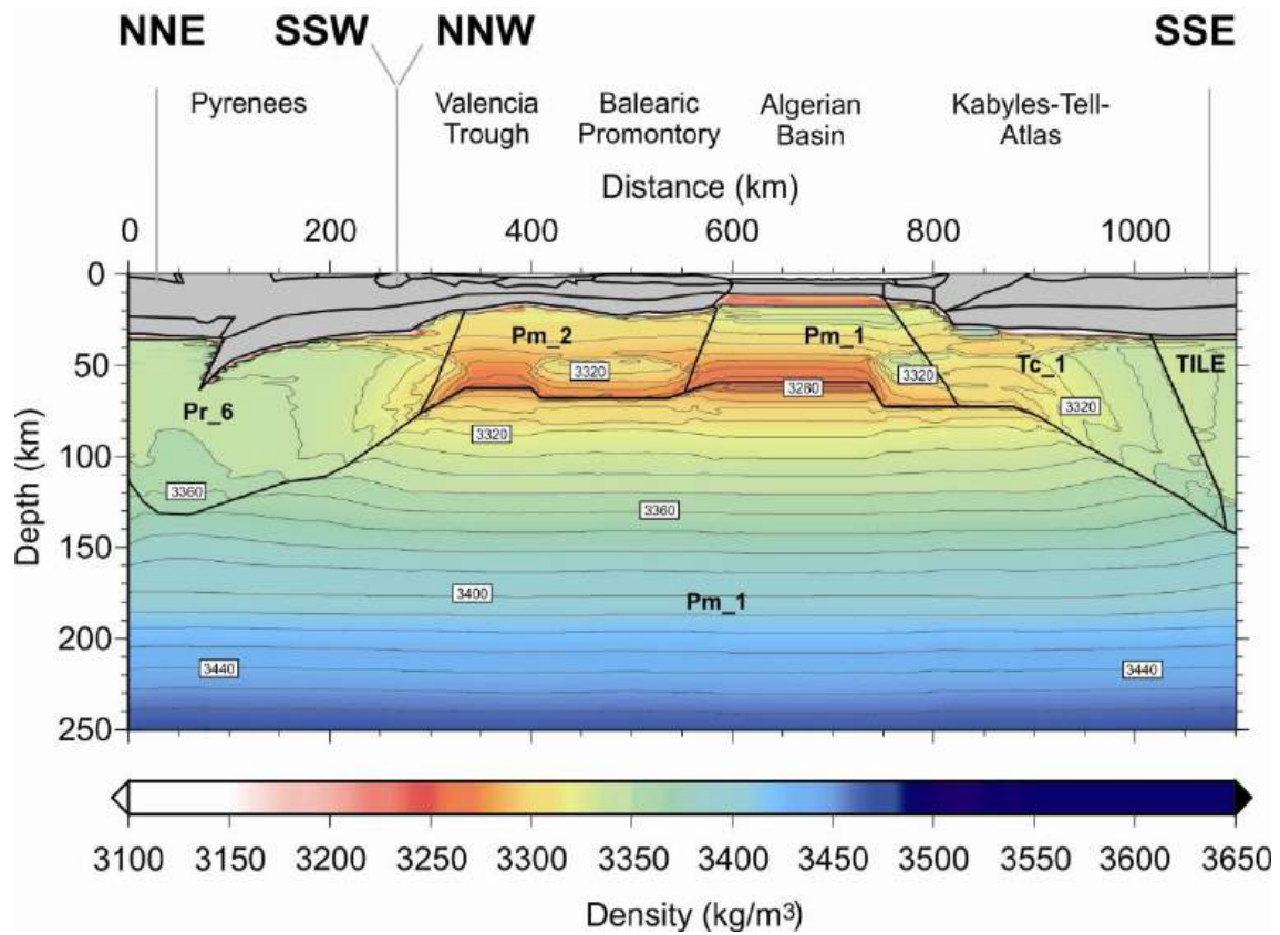
Figure 2.7: Calculated mantle density distribution along the modeled transect. Contour lines every 10 kg m -3 . Sharp density increase in the uppermost mantle beneath the Algerian Basin is related to the Pg-Sp phase transition. Sharp density increase at ~50 km depth is related to Sp-Grt phase transition.
