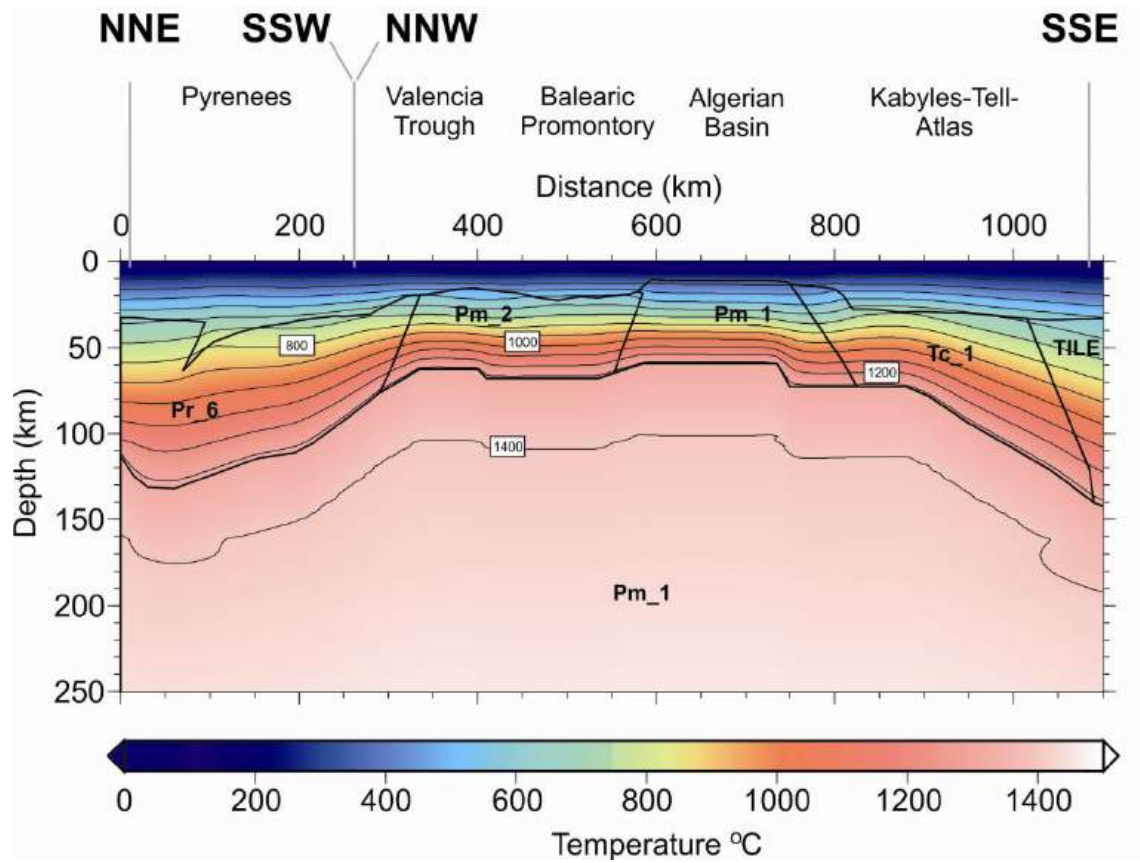
Figure 2.6: Calculated temperature distribution along the modeled transect. Contour lines every 100 °C.
