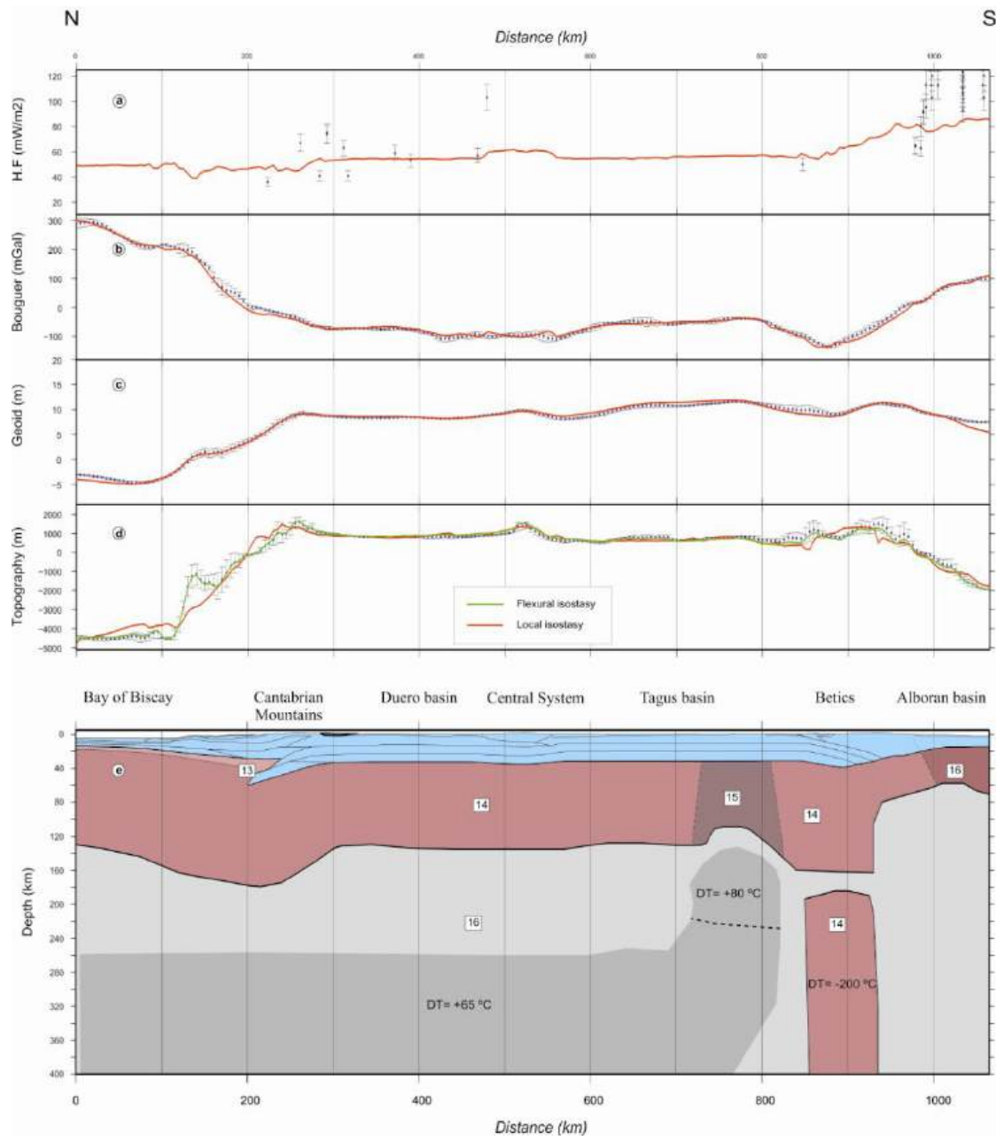
Figure 4.4: Model results (red lines), measured data with the standard deviation of data projected onto the profile within a strip of 25 km half-width (blue dots and vertical bars), coupled calculated topography (red line), and green line represent calculated elevation in the case of effective elastic thickness for the different T_e (30 km, 20 and 10 km) used along the profile (see text for details): (a) surface heat flow; (b) Bouguer anomaly; (c) geoid height; (d) elevation; (e) lithospheric structure. Crustal structure like in Figure 4.2. Numbers in panel (e) denote mantle bodies summarized in Table 4.1. Dataset sources as in Figure 1.3.
