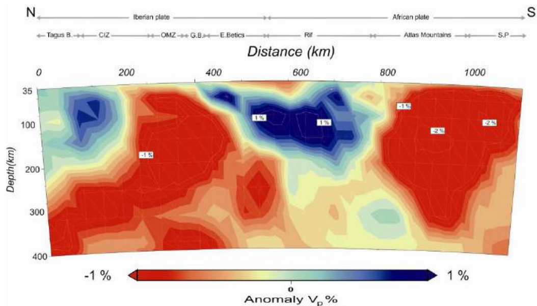
Figure 5.3: P-wave tomography model along the Iberian Massif-Arc of Gibraltar-Atlas Mountains (fourth profile) based on the global travel-time tomography model of Villaseñor et al. (2003).
