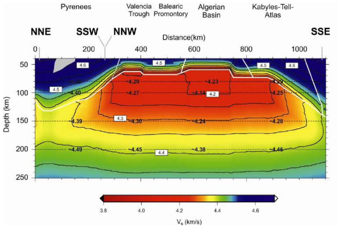
Figure 2.9: Calculated S-wave seismic velocities in the upper mantle (calculations extend down to 400 km depth). White solid lines indicate mantle domains with different chemical composition. Contour lines every 0.05 km/s. Superimposed are the S-wave velocities inferred from the regional tomography model by Legendre et al. (2012) at different depth levels. S-values have been calculated according to the reference velocities of 4.38 km/s (at 80 and 110 km), 4.39 km/s (at 150 km) and 4.45 km/s (at 200 km) (see Legendre et al., 2012).
