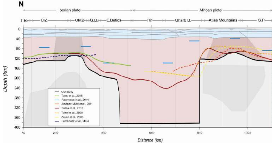
Figure 5.11: Calculated topographies of the lithosphere-asthenosphere boundary from different models. Dashes lines correspond to profiles that not coincide with the direction of the Iberian Massif-Arc of Gibraltar-Atlas Mountains geo-transect. CIZ, Central Iberian Zone; OMZ, Ossa Morena Zone; GB, Guadalquivir Basin; S.P, Sharan Platform.
