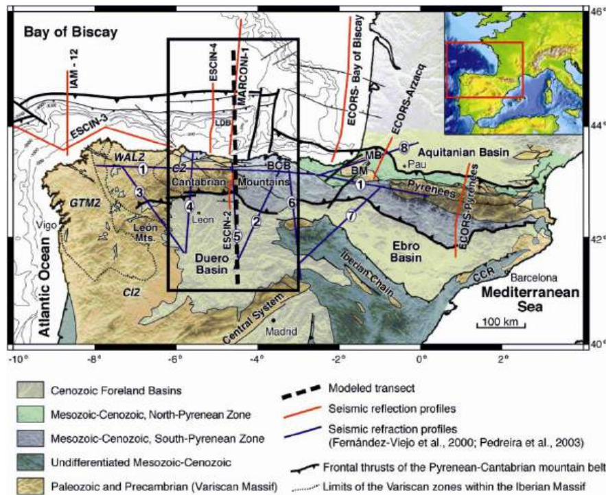
Figure 3.1: Tectonic map of the Pyrenean-Cantabrian mountain belt in north-Iberia showing the location of the modeled N-S lithospheric transect and available deep seismic profiles. BCB, Basque-Cantabrian basin; BM, Basque Massifs; CCR, Catalan Coastal Ranges; MB, Mauléon basin. Acronyms in italics refer to tectonometamorphic zones within the Iberian Variscan Massif: CIZ, Central Iberian Zone; CZ, Cantabrian Zone; GTMZ, Galicia – Tras os Montes Zone; WALZ, West Asturian-Leonese Zone.
