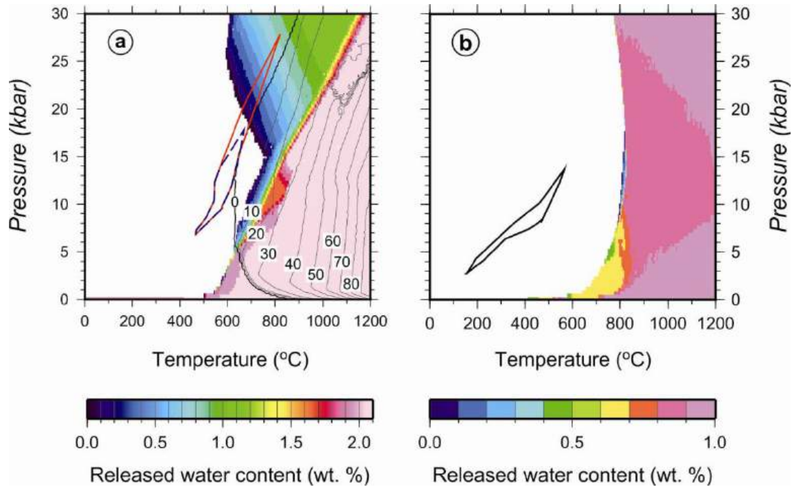
Figure 6.4: Schematic illustration of the water balance between the dehydrated subducting lower crust and the overlying hydrated mantle wedge. a) In colors: released water (in wt. %) of the subducting Iberian lower crust calculated using Perple_X (Connolly, 2009; 2005) according to the “intermediate” composition listed in Table 2.2. In black contours: percentage of partial melt for the same composition, according to the model of Holland and Powell (2001) and White et al. (2001). The superimposed blue and red outlines mark the pressure-temperature conditions for the piece of Iberian lower crust with that composition, for model. b) Same type of diagram but for the body of hydrated upper mantle, with 1 wt.% of \text{H}_2\text{O} in its composition (Table 2.2). As observed, this body keeps the 100% of the structural water unless heated up to more than \sim 700^\circ\text{C} .
