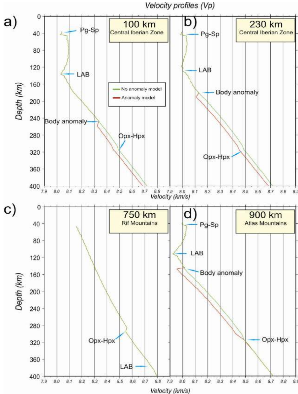
Figure 5.12: Depth variation of P-wave velocities calculated in the preferred model along the profile (in sites located at 100, 230, 750 and 900 km horizontal distance) for model with the sub-lithospheric anomalous body (red line) and model without the anomalous body (green line). Arrows denote the lithosphere-asthenosphere boundary (LAB) and the following phase transitions: Pg-Sp, plagioclase-spinel; Opx-Hpx, orthopyroxene-high-pressure magnesian pyroxene.
