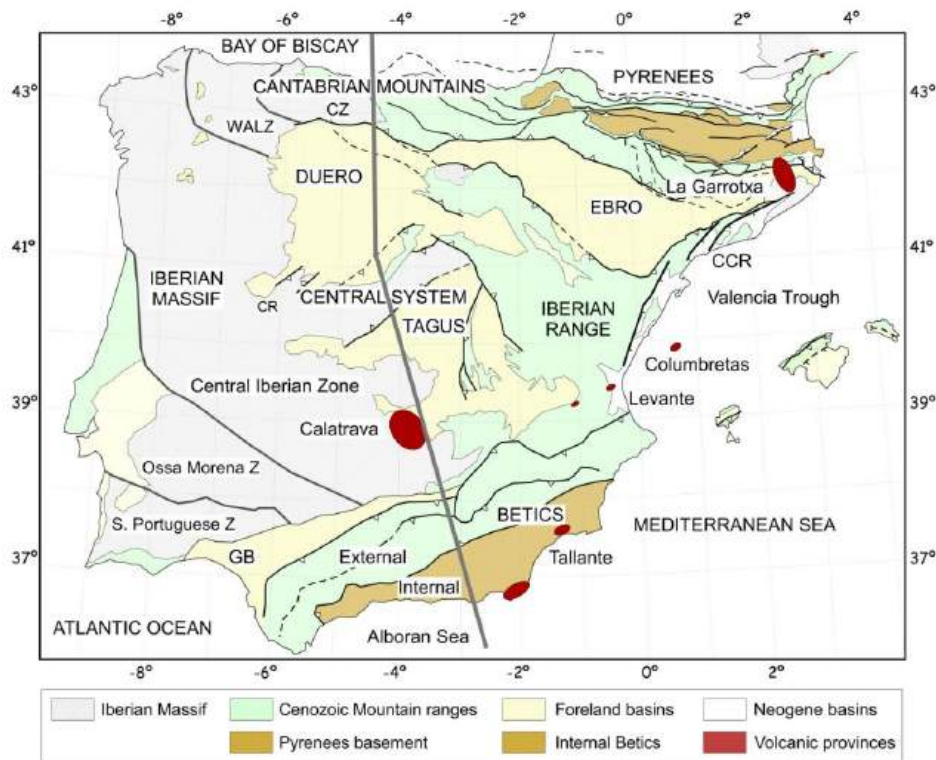
Figure 4.1: Geological map of the study area showing the principal geological domains of Iberia (modified after Vergés and Fernández, 2006). Thick gray line locates the modeled transect.
