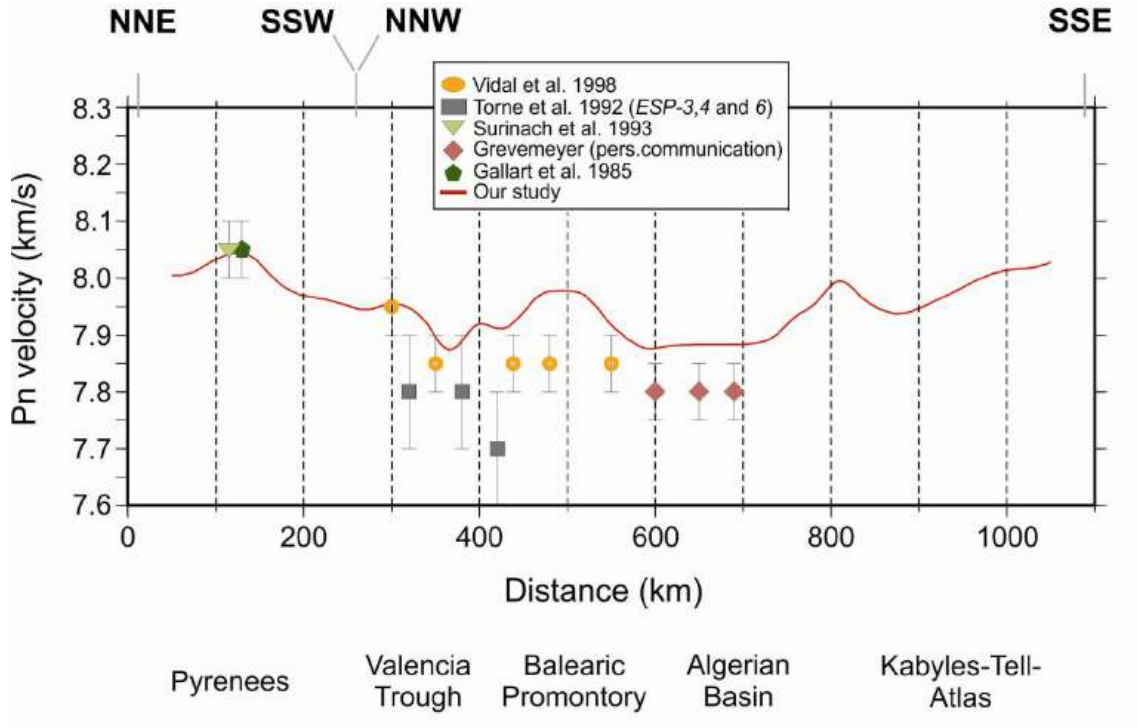
Figure 2.10: Pn velocities along the modeled transect. Red line indicates calculated Pn values. Symbols with error bars denote Pn-values from seismic experiments (see legend).
