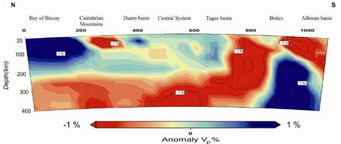
Figure 4.3: P-wave tomography model along the Cantabrian Mountains–Central System–Betics geotranssect (third profile) based on the global travel-time tomography model of Villaseñor et al. (2003).
