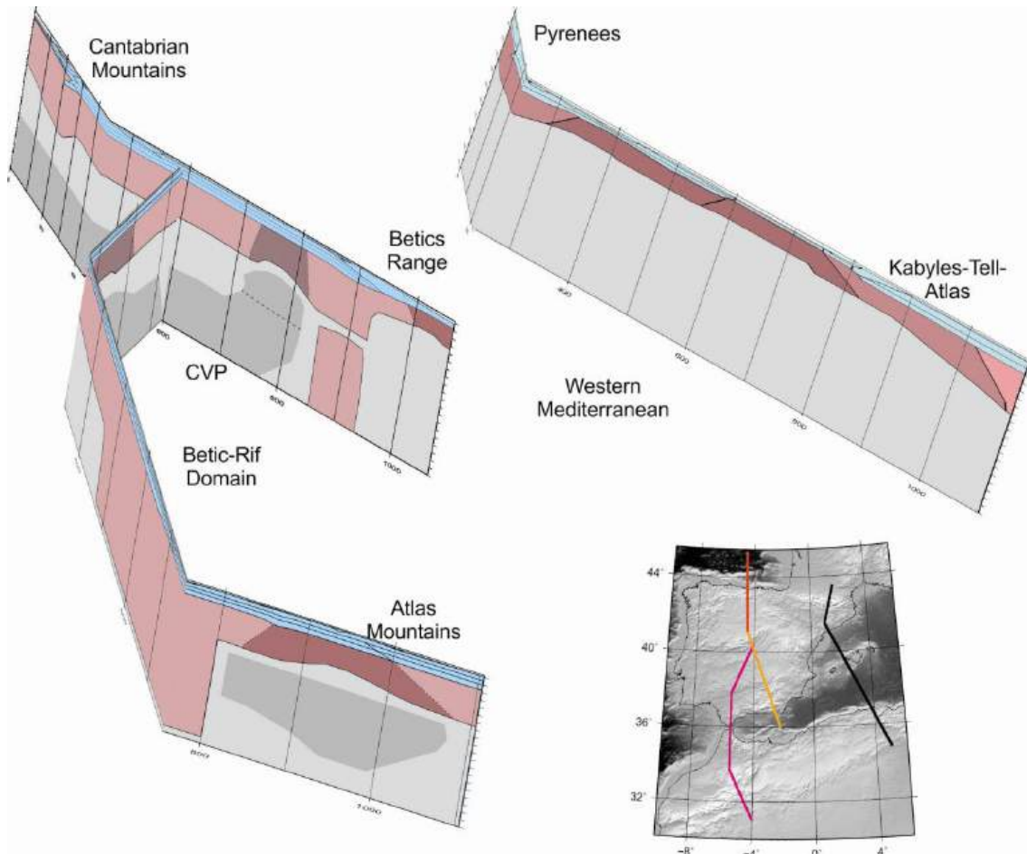
Figure 6.1: Schematic crust and upper mantle cross-sections of Iberia and North Africa of the four modeled geo-transects (second geo-transect is integrated in the third lithosphere profile). Lower right inset shows the location of the fourth geo-transects in the study area.
