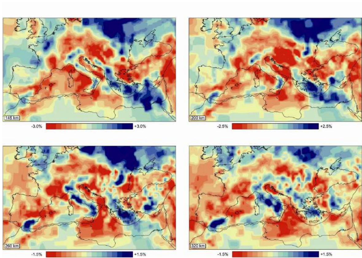
Figure 1.2: P-wave anomaly of the western-Mediterranean region from the tomography model of Villaseñor et al., 2003 for different depths (145, 200, 260 and 320). Shown are P wave seismic velocity anomalies relative to the 1-D reference model ak135 of Kennett et al. (1995). The blue anomaly under the Rif-Gibraltar-Betic (RGB) (southern Iberia) is the image of the slab. Courtesy by A. Villaseñor.
