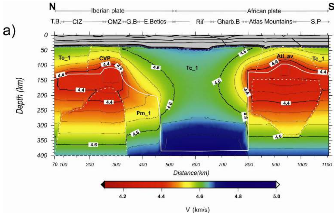
Figure 5.9: Calculated S-wave seismic velocities in the upper mantle down to 400 km depth. Contour lines every 0.05 km/s.
