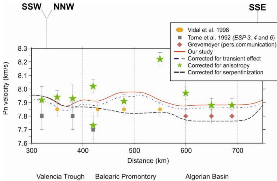
Figure 6.3: Pn velocities along the W-Mediterranean segment of the modeled transect. Circles with error bars denote Pn values from seismic experiments (see Fig. 3.10 for data sources). Red solid line denotes calculated values from our model. Stars with error bars denote Pn values from seismic experiments corrected for anisotropy effects. Blue dotted line denotes calculated values corrected for thermal transient effects. Stippled black line denotes calculated values incorporating serpentinization. See text for details.
