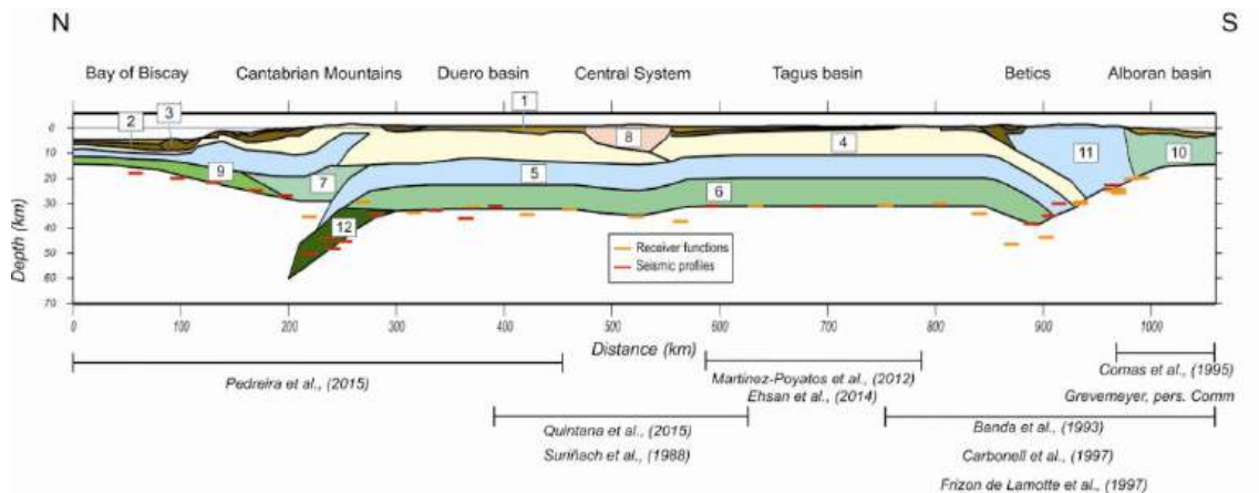
Figure 4.2: Crustal structure corresponding to the best fitting model. Different bodies have been modeled using geological cross-sections (overlaid) and seismic experiments (see text for details). Physical properties of crustal bodies are reported in Table 4.1.
