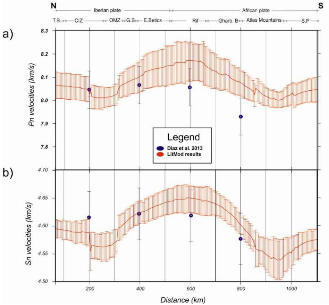
Figure 5.10: a) Pn velocities along the modeled transect. Red line indicates calculated Pn values. Circles with error bars denote Pn-values from seismic experiments (see legend); b) Sn velocities along the modeled transect. Red line indicates calculated Sn values. Symbols with error bars denote Sn-values from Diaz et al. (2013).
