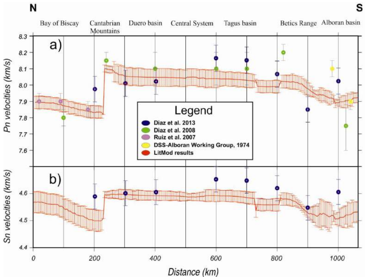
Figure 4.9: a) Pn velocities along the geo-transect. Red line indicates calculated Pn values with the associated standard deviation of the first 15 km of the uppermost mantle. Circles with error bars denote Pn-values from seismic experiments (see legend); b) Sn velocities along the modeled transect. Red line indicates calculated Sn values. Symbols with error bars denote Sn-values from Diaz et al., 2013.
