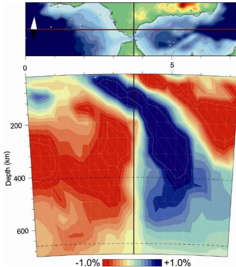
Figure 5.5: East to west tomographic cross-section based on the tomographic model of Villaseñor et al. (2003). Black line shows the location of the Iberian Massif-Arc of Gibraltar-Atlas Mountains geo-transect.
