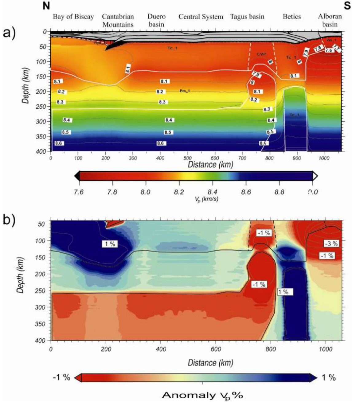
Figure 4.7: a) Calculated P-wave seismic velocities in the upper mantle down to 400 km; b) synthetic P-wave tomography from our model. In this case velocity anomalies are relative to the synthetic reference model (calculated from V_p in (%) relative to a reference model consisting of a 130 km thick lithosphere and 30-km thick crust with a lithosphere mantle composition corresponding to Tc_1) (see text). Contour lines every 1%. Compare with Figure 4.3.
