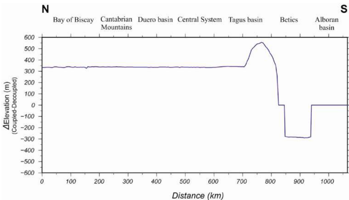
Figure 4.13: Difference between the elevations calculated considering coupled and decoupled anomalous sub-lithospheric bodies.
