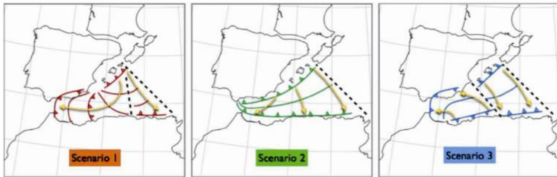
Figure 1.4: An illustration of rollback as portrayed in the three different reconstruction scenarios from Chertova et al., 2014. Scenario 1 (Spakman and Wortel, 2004) and scenario 2 (Faccena et al., 2004) assume a unique subduction polarity but start from different initial subduction zone (short and long respectively). Scenario 3 (Vergés and Fernandez, 2012) shows two opposite dipping subductions. Dashed lines represent proposed transform fault regions. The triangular zone between the transform zones of Scenario 1 depicts the lithosphere that rolls back toward the east Kabyliides (Spakman and Wortel, 2004).
