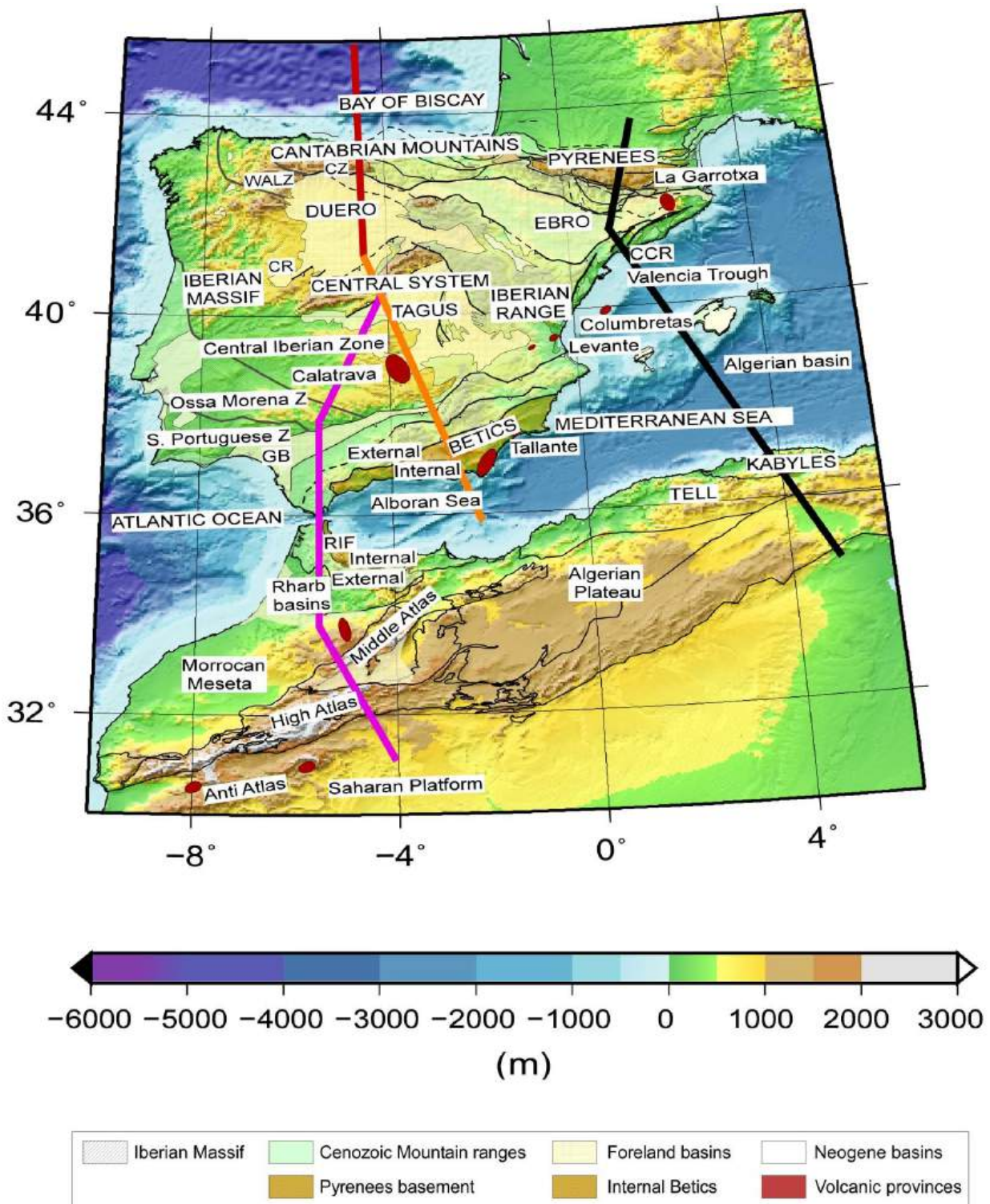
Figure 1.1: Geological map of the study area showing the principal geological domains of Iberia and North Africa. Thick lines locate the modeled transects: Black line-first geo-transect; Red line-second geo-transect; Orange line-third geo-transect and pink line-fourth geo-transect. WALZ, west Asturian-Leonese Zone; CZ, Cantabrian Zone; CCR, Catalan Coastal Ranges; CR, Ciudad Rodrigo Basin, located in the SW side of the Duero Basin; GB, Guadalquivir Basin.
