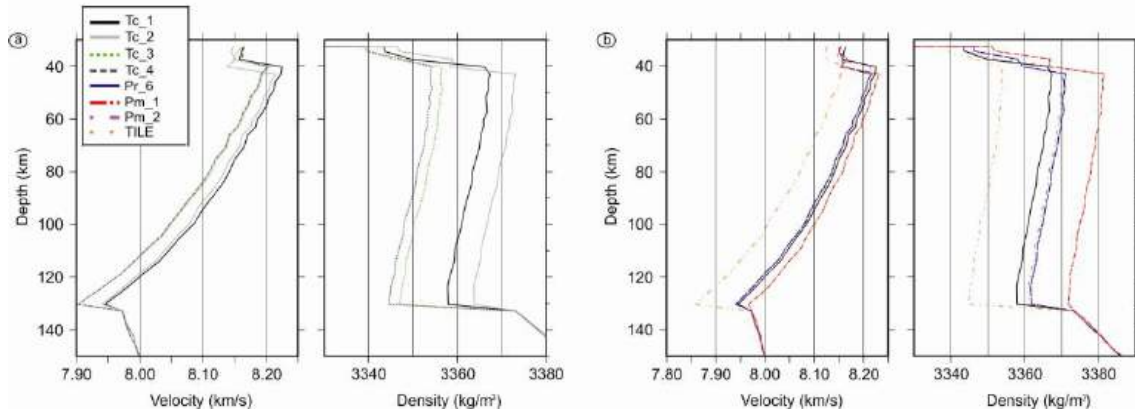
Figure 2.11: a) Depth variation of P-wave velocities (left panel) and densities (right panel) calculated for different average-Tecton mantle compositions according to Griffin et al. (2009) for a 1-D lithosphere structure consisting of 32 km thick crust and 130 km thick lithosphere. b) Same as a) for the mantle chemical compositions used in our modeled transect (see Table 2.2).
