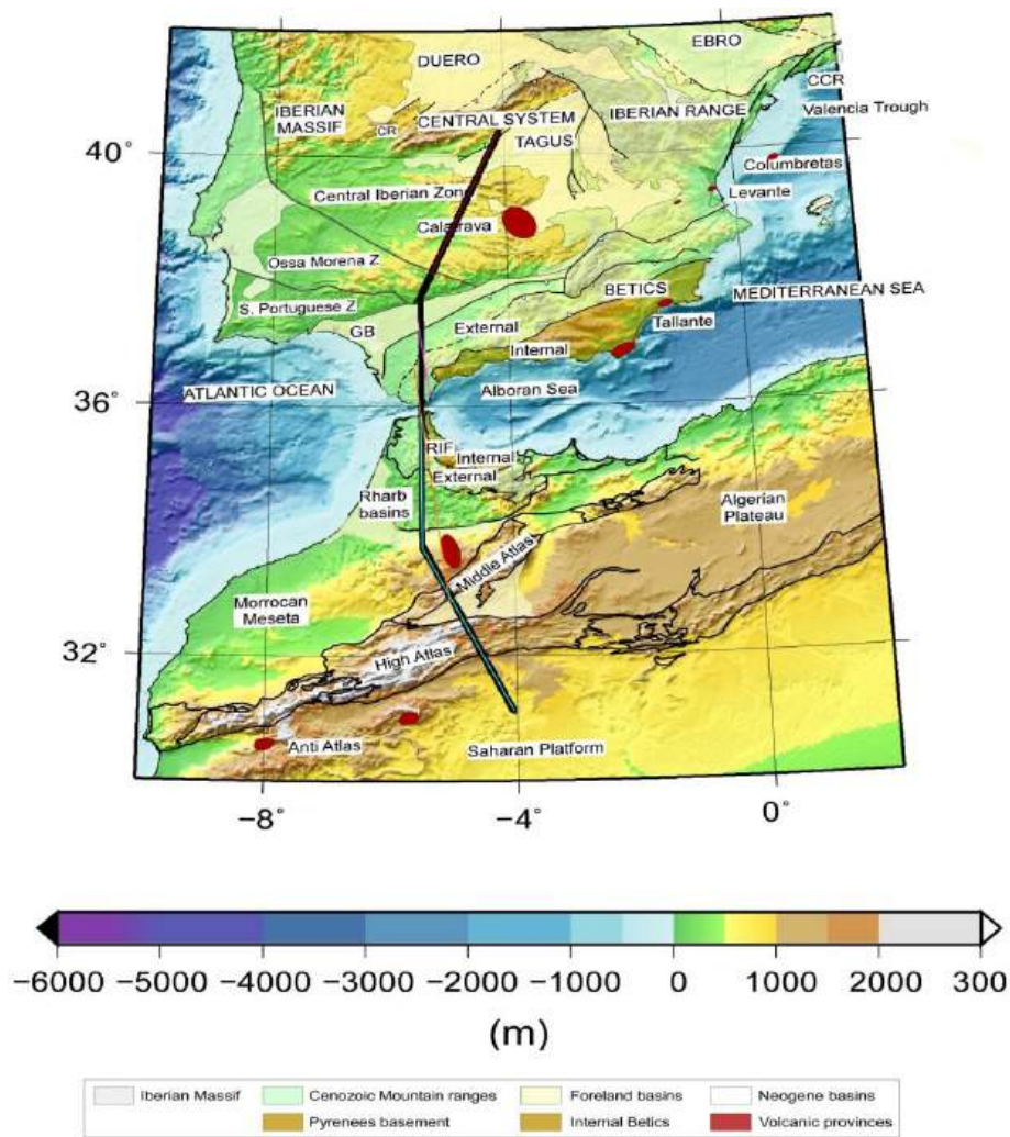
Fig. 5.1: Geological map of the study area showing the principal geological domains of the study area. Thick black line locates the modeled transect. Thin lines locates the seismics experiments: Red line- ALCUDIA wide-angle (Ehsan, 2014); Pink line- La Línea-Carmona (Medialdea et al., 1986); RIFSIS wide-angle (Gil et al., 2014); and SIMA wide-angle (Ayarza et al., 2014).
