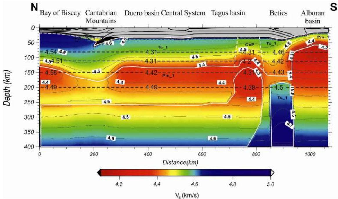
Figure 4.8: Calculated S-wave seismic velocities in the upper mantle down to 400 km depth. Contour lines every 0.05 km/s. Superimposed are the S-wave velocities inferred from the regional tomography model by Legendre et al. (2012) at different depth levels. S- values have been calculated according to the reference velocities of 4.38 km/s (at 80 and 110 km), 4.39 km/s (at 150 km) and 4.45 km/s (at 200 km) (see Legendre et al., 2012).
