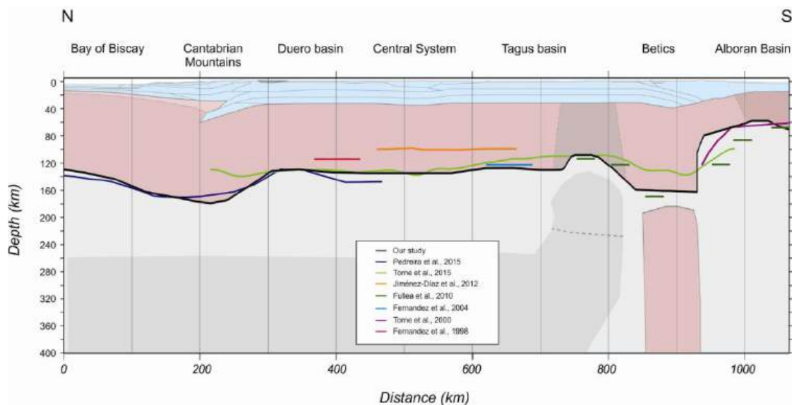
Figure 4.10: Calculated topographies of the lithosphere-asthenosphere boundary from different models.
