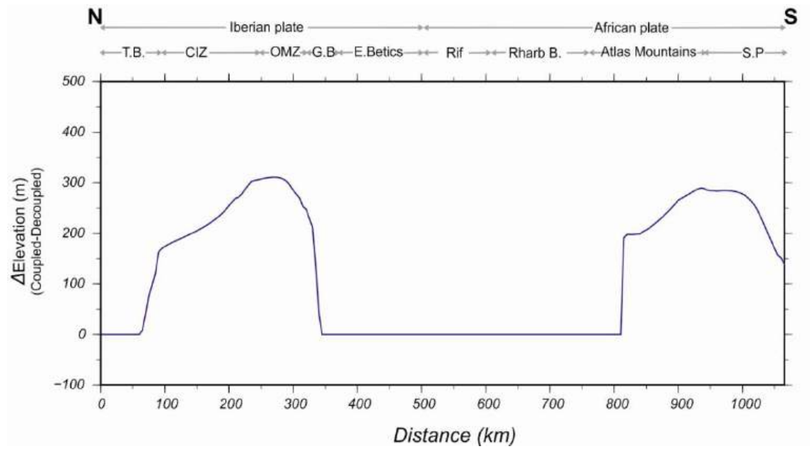
Figure 5.14: Difference between the elevations calculated considering coupled and decoupled anomalous sub-lithospheric bodies.
