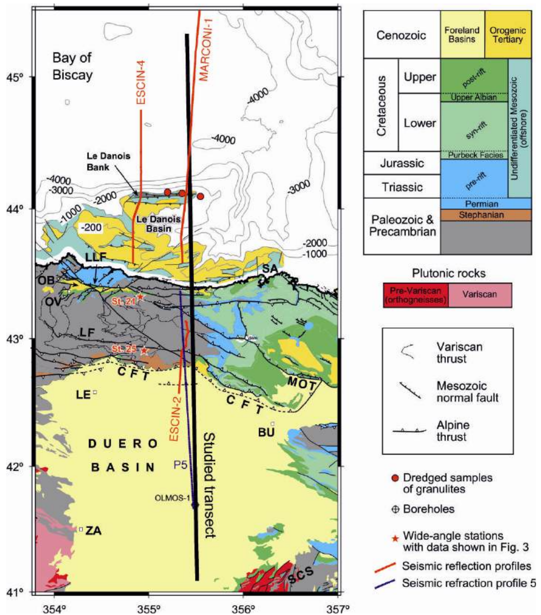
Figure 3.3: Detailed geological map of the investigated transect, modified from previous synthesis by Alonso et al. (1996), Quintana (2012), Rodríguez Fernández et al. (2004) and Gallastegui et al. (2002). Cities: BU, Burgos; LE, León; OV, Oviedo; SA, Santander; ZA, Zamora. Geological features: CFT, Cantabrian Frontal Thrust; LF, León Fault; LLF, Llanera Fault; MOT, Montes Obarenes Thrust; OB, Oviedo Basin; SCS, Spanish Central System.
