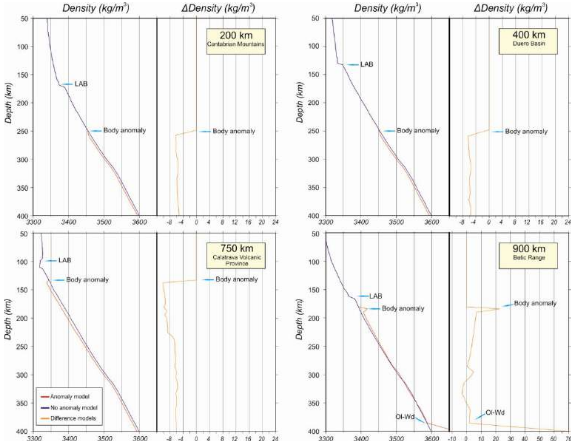
Figure 4.12: Depth variation of mantle density calculated in the preferred model along the profile (at 200, 400, 750 and 900 km distance) for model with asthenospheric anomaly and model without asthenospheric anomaly.
