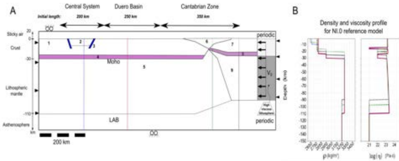
Figure 4.3. A) Reference model (N1.0) geometry showing the layering thickness of the different bodies which densities and viscosities are listed in Table 4.1. Constant velocity of 2.5 mm/y, it is an indentation of a high viscous mantle of 10^{24} Pa·s without plasticity criterion to prevent high deformation. B) Density and viscosity profiles of four different sections of the reference model (dashed lines Figure 4.3A). Note that the viscosity profile corresponds to values in the model and is computed based on a constant strain rate ( 10^{-15} s^{-1} ). Vertical axis is exaggerated.
