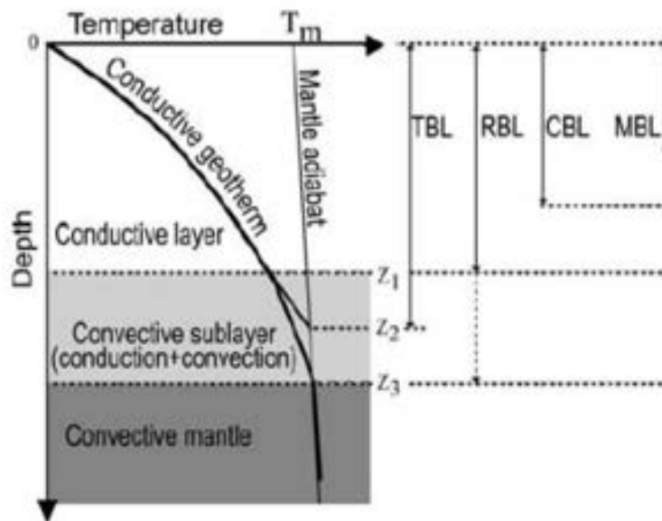
Figure 2.1. Scheme of the 4 accepted definitions of the Lithosphere-Asthenosphere Boundary (LAB). TBL, RBL, CBL, and MEL are the thermal, rheological, chemical and mechanical boundary layers. Above Z_1 the layer has only conductive heat transfer. Z_2 is representative of the TBL where a linear geotherm intersect the mantle adiabetic or solidus temperature. These definitions (except chemical boundary layer) are temperature-dependent where a dramatic change in mantle viscosity occurs. Modified from Artemieva (2011).
