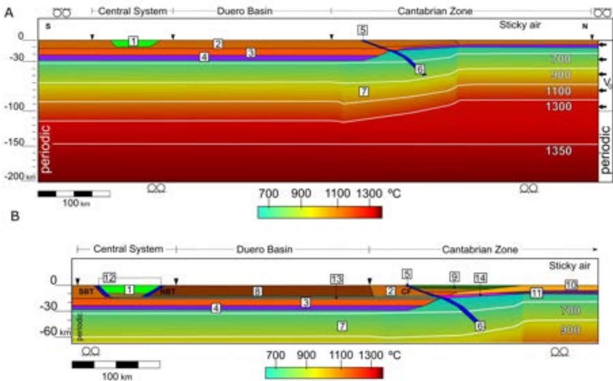
Figure 4.9. A) Set-up for the reference model (TM0). B) Set-up for the last model (TM4). Material numbers correspond to materials listed in Table 4.3. V_0 is the initial velocity of 2.5mm/y. White lines are temperature contour for the lithospheric mantle in Celsius. Black triangles of the surface correspond to the location of the upper crust markers in order to calculate shortenings for the 3 different sectors; Central System, Duero Basin and Cantabrian Zone. NBT: North Boundary Thrust and SBT:South Boundary Thrust
