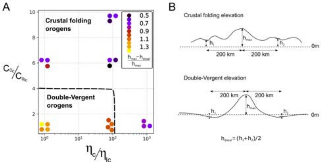
Figure 5.1. A) Overview of all models comparing crust and lower crust cohesion ratio vs. initial viscosity ratio when reaching 100 km of crustal shortening. The colour scale represents relieve: the difference between the maximum and the average value of a distal elevation divided by the maximum elevation of the orogen. Double-vergent (DV) models correspond to values above 1. B) Schematic clarification to calculate the relieve shown in colours in A. h_1 and h_2 are the average (among the particles inside a cell) elevations at 200 km from the center of the orogen (higher elevation).
